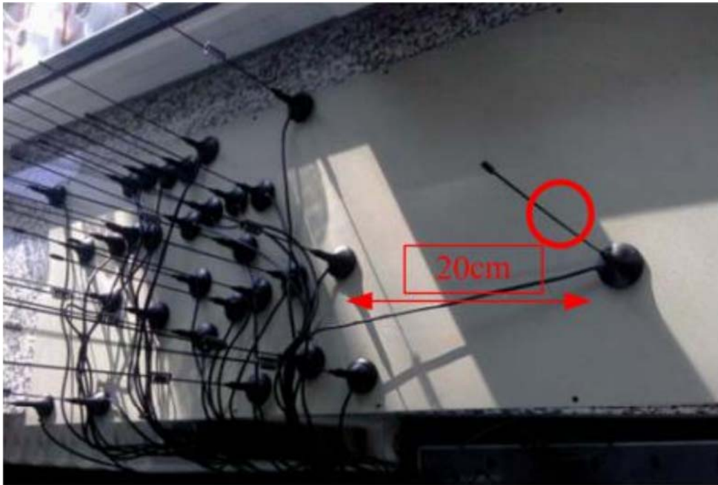
figure-6.1 Theoretic distance value for GSM band
