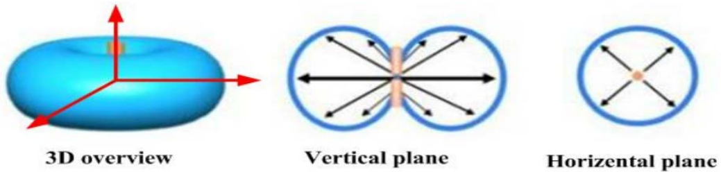
Radiation pattern of low directivity antenna
