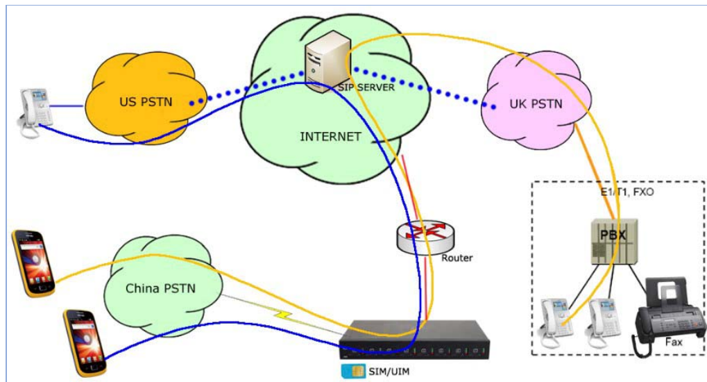
Figure 1-2-1 Network scenario
