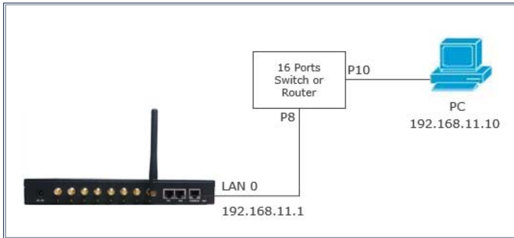
Figure 2-2-5DVG-6008G networkconnection
