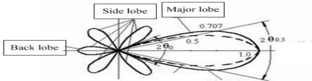
radiation pattern of high directivity antenna
