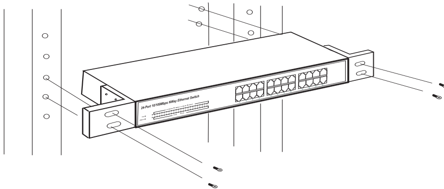
Installing the Switch in an equipment rack
