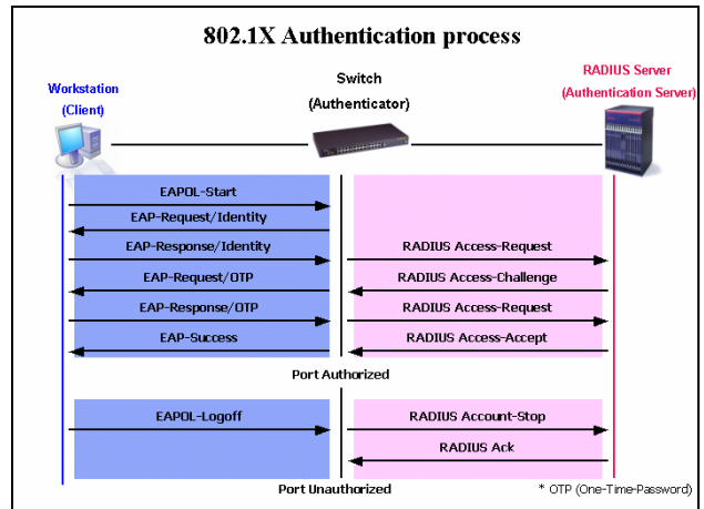
Figure 10-6 The 802.1X Authentication Process
