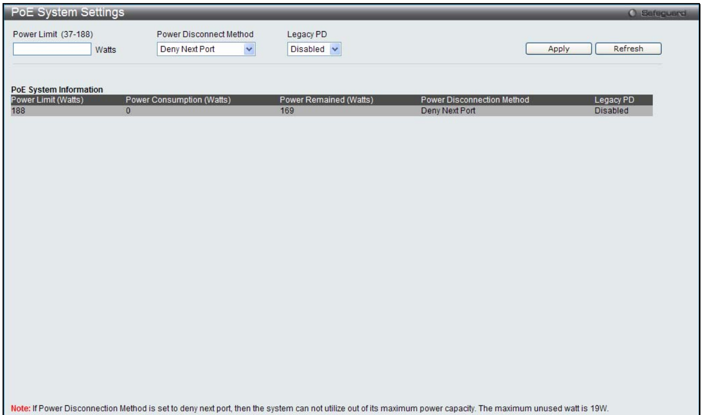
Figure 2-14 PoE System Settings window
