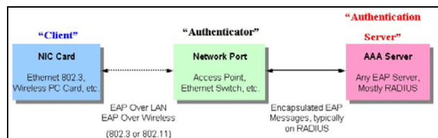
Figure 10-2 The three roles of 802.1X
