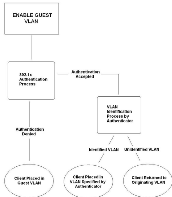
Figure 10-12 Guest VLAN Authentication Process
