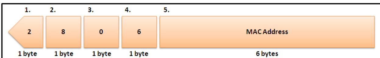
Figure 11-3 Remote ID Sub-option Format
