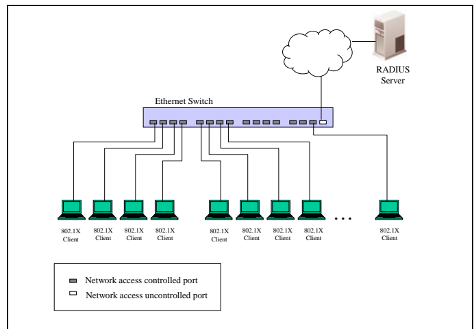
Figure 10-7 Example of Typical Port-based Configuration
