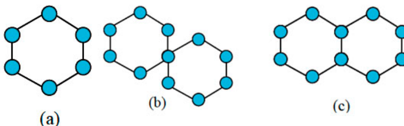
Figure 4-80 Ethernet ring topologies supported by ERPS
