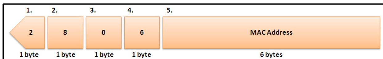
Figure 9-3 Remote ID Sub-option Format
