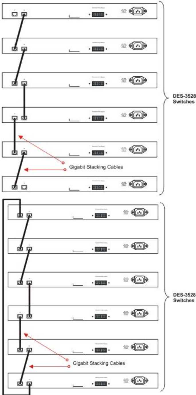
Figure 2-26 Switches stacked in a Duplex Chain
