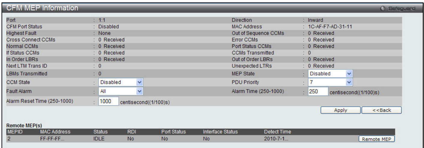
Figure 10-6 CFM MEP Information - Edit window
