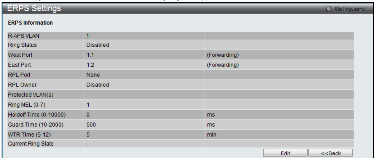
Figure 4-82 ERPS Settings - Detail Information window
