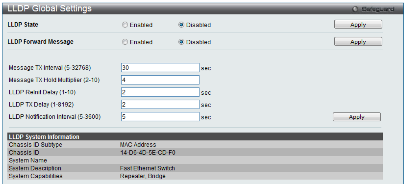
Figure 4-84 LLDP Global Settings window
