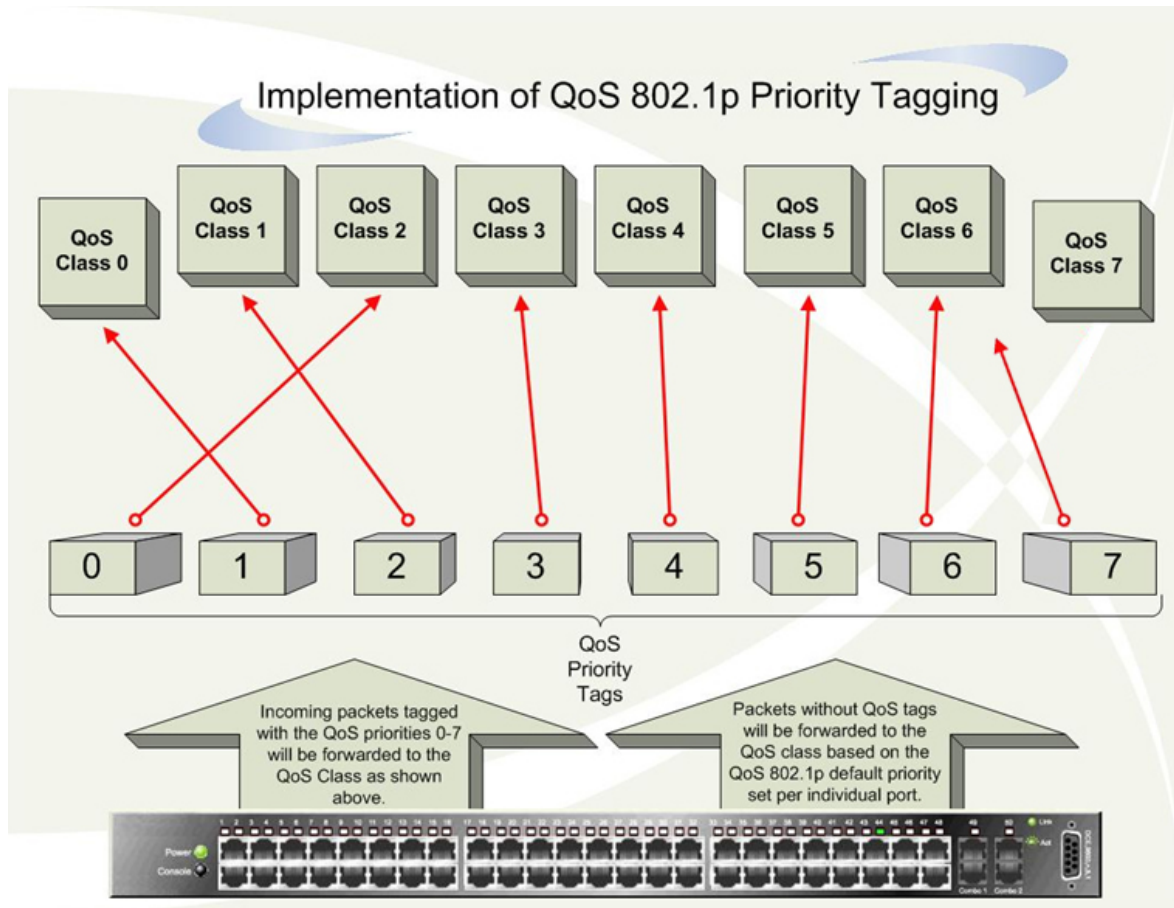
Figure 6-1 Mapping QoS on the Switch
