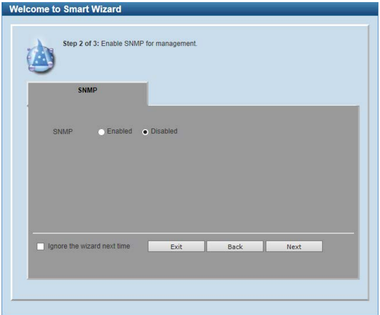
Figure 2-4 SNMP window
