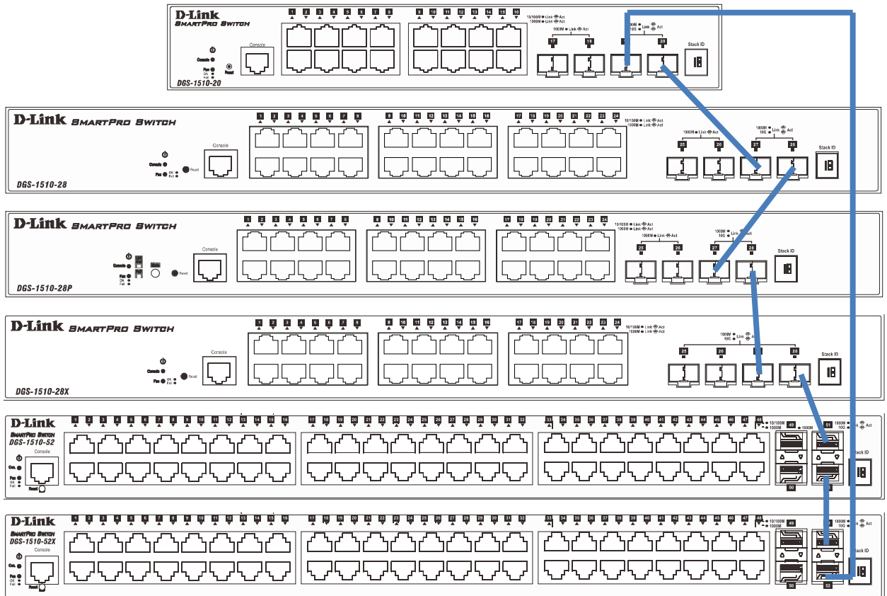
Figure 4-46 Switches stacked in a Duplex Ring
