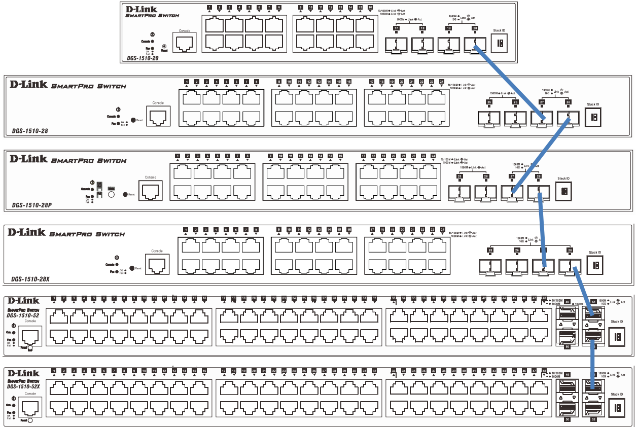
Figure 4-45 Switches stacked in a Duplex Chain
