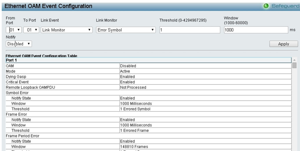
Figure 4.93 - Configuration > Ethernet OAM > Ethernet OAM Event Configuration
