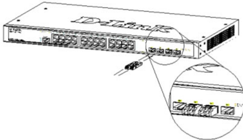
Figure 1-11. Inserting the SFP modules into the Switch
