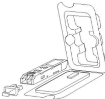
Figure 1-12. Installing the SFP Module
